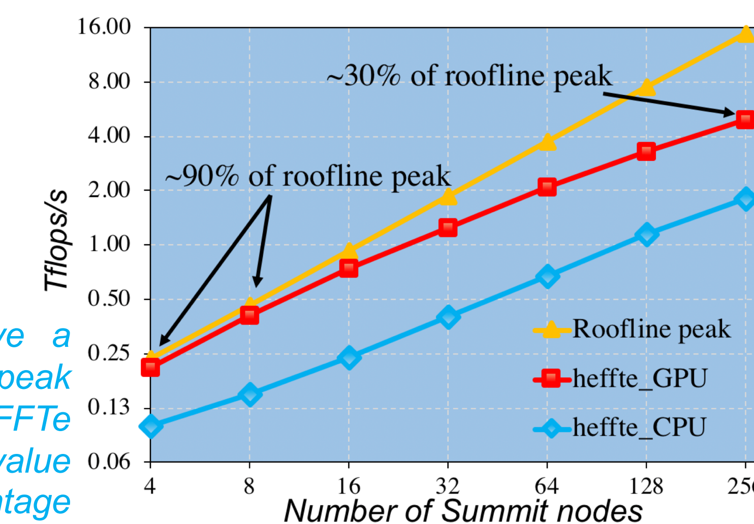
Fig 4. Roofline & scalability for heFFTe , GPU version uses 6 Volta100 GPUs per node, CPU version uses 40 IBM Power9 per node.
