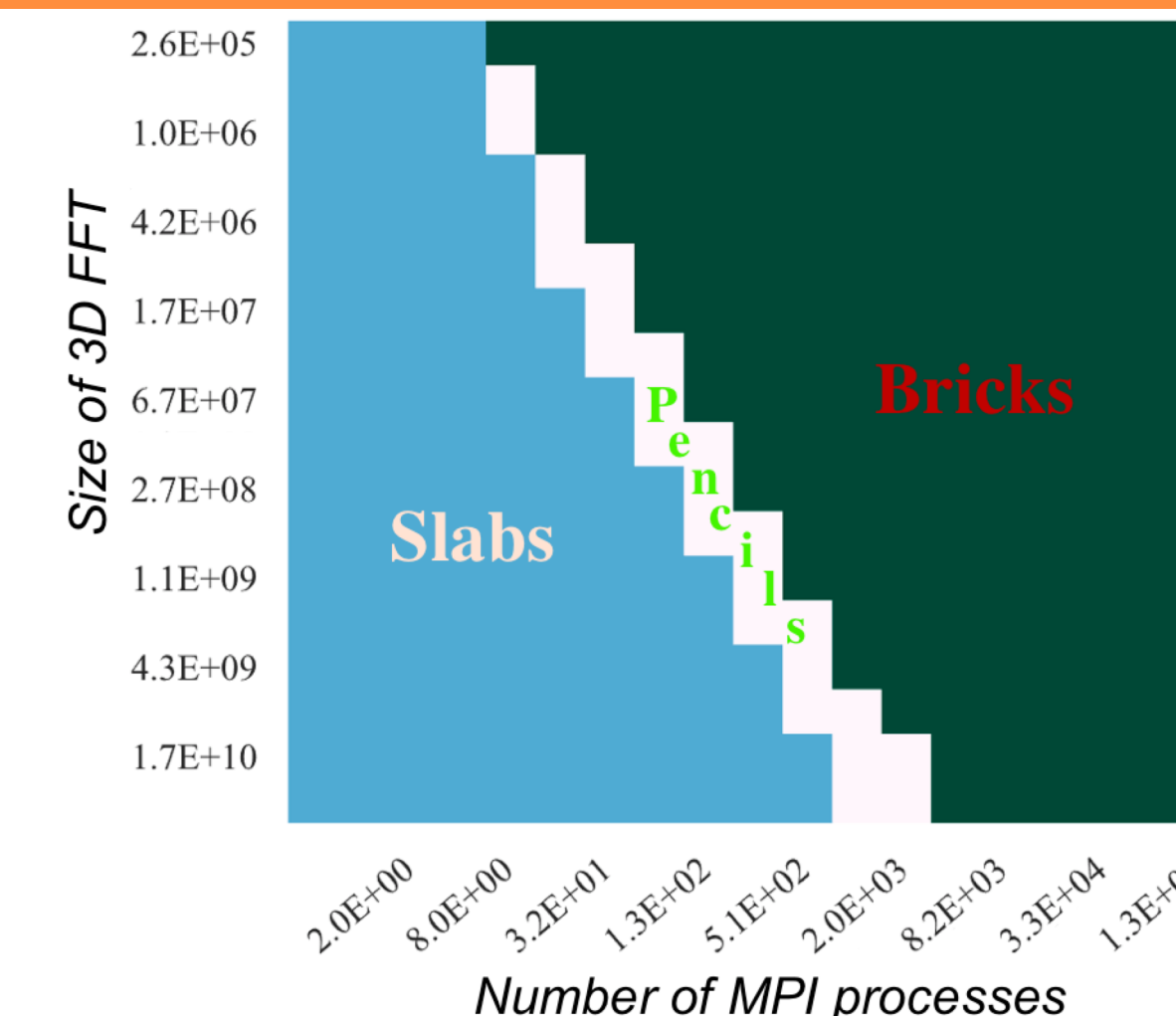
Fig 2.2. Phase diagram for algorithm tuning
