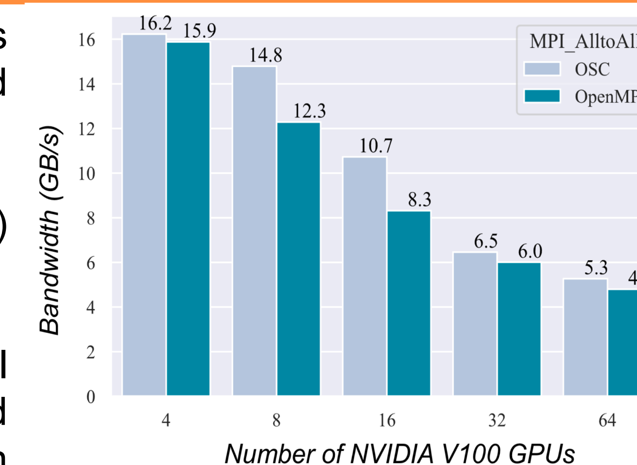
Fig 2.3. Average throughput of all-to-all exchange of 2GB of data, 1GPU per node.
