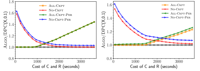
(a) Exponential (Mean: 3600s) (b) Bounded Pareto (Mean: 6630s)
