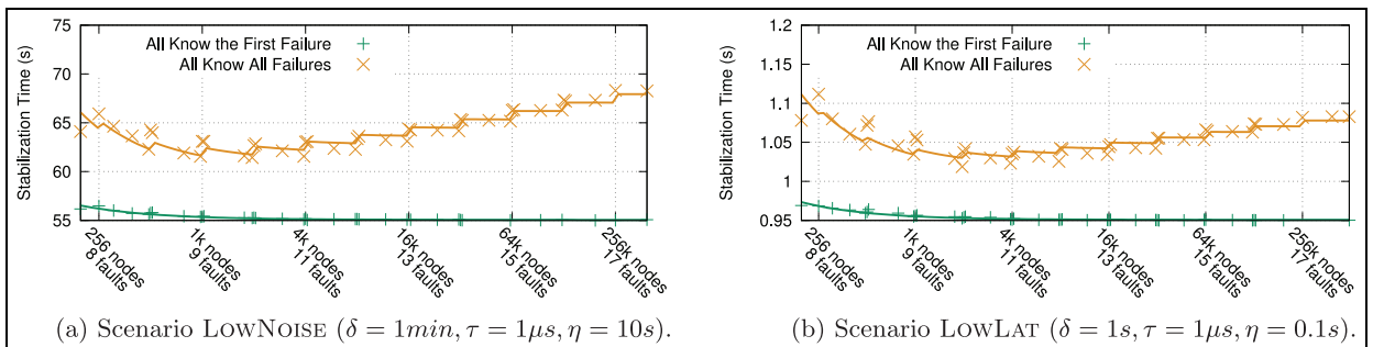
Figure 4. Average stabilization time, when the maximal number of failures strike a platform of varying size.
