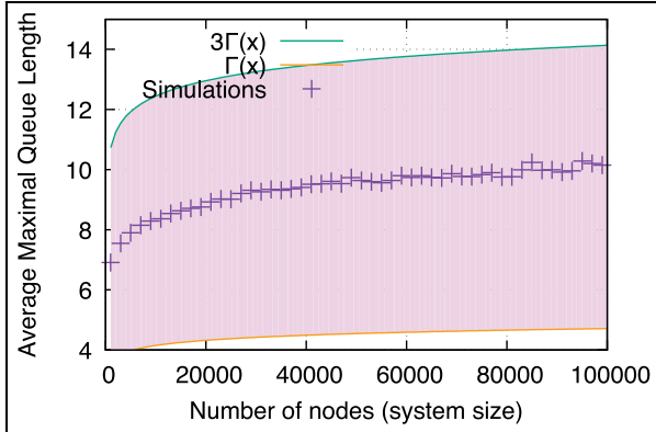
Figure 7. Average of the maximum length of queue size L(N) during a single round, for the randomized ping protocol.
