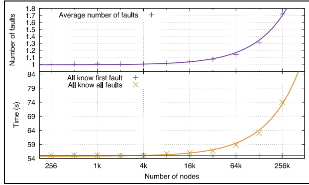
Figure 5. Average stabilization time, with random overlapping failures in scenario LowNOISE ( \delta = 1 min, \tau = 1 \mu s, \eta = 10 s), with \mu_{\text{ind}} = 1 year.
