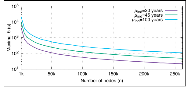
Figure 3. Maximal value for \delta to ensure that P_{T(M)}(M) < 10^{-9} with \tau = 1 \mu\text{s} and M = \lfloor \log_2(n) \rfloor .
