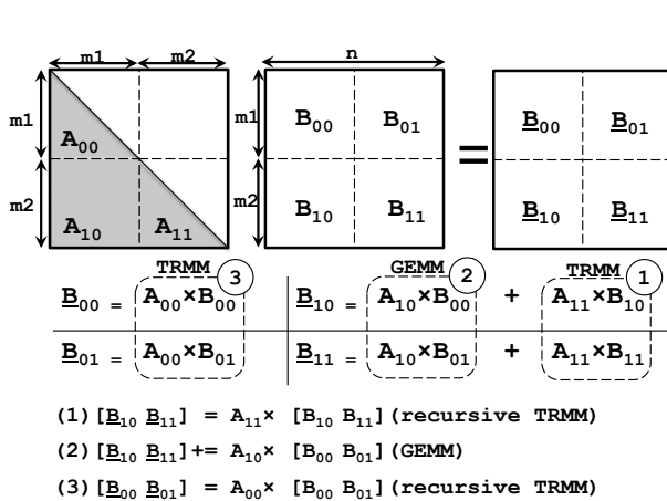
Figure 7: TRMM design.
