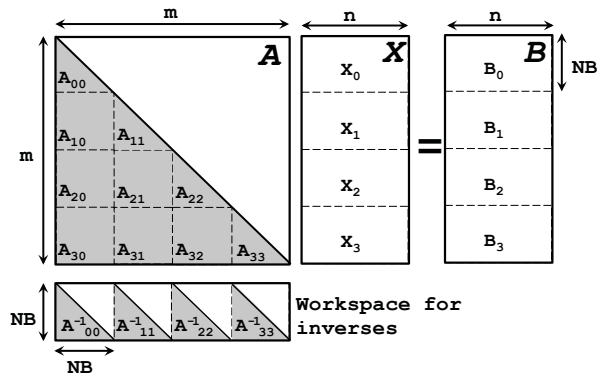
Figure 8: TRSM design.
