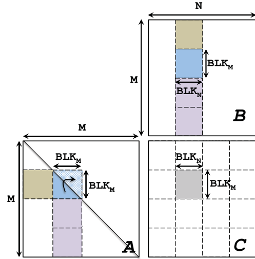
Figure 5: HEMM design.
