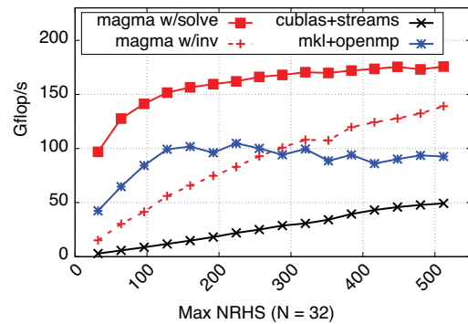
(b) Solve X_{m \times n} \cdot A_{n \times n} = B_{m \times n} , ( n = 32 )
