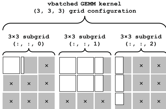
Figure 2: Example of vbatched GEMM using ASGT.
