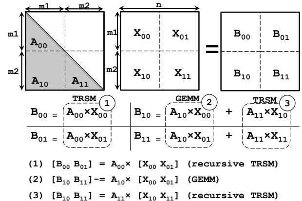
Figure 11: TRSM design.
