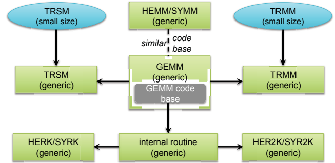
Figure 3: Overall design of BLAS-3 routines.
