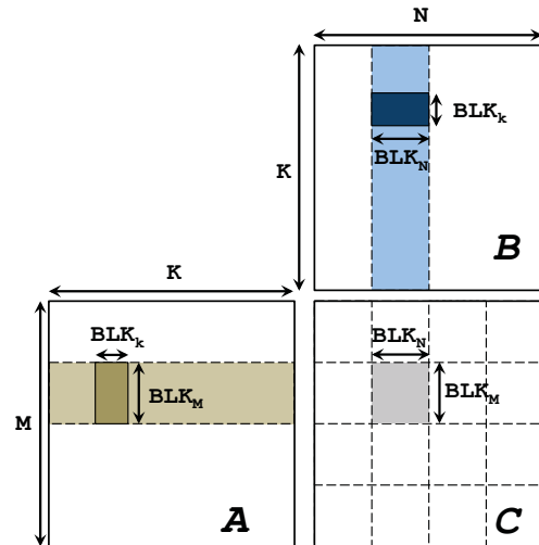
Figure 4: GEMM design.
